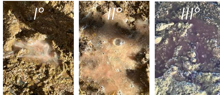
Metrite # Endometrite
