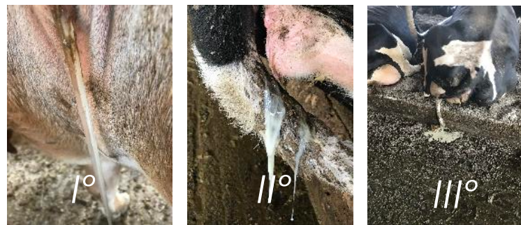
Metrite # Endometrite
